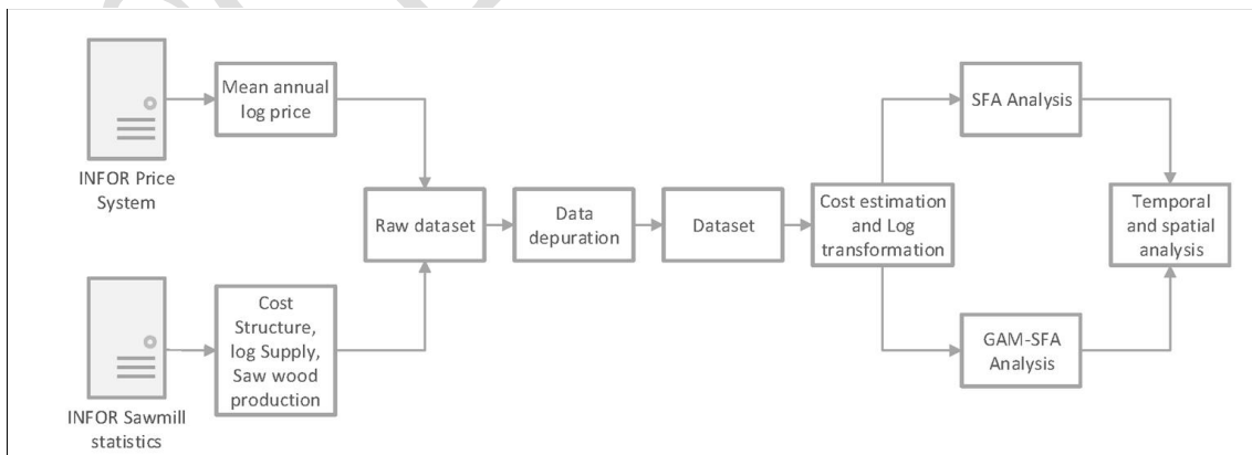
Figure 1: Methodology diagram.
