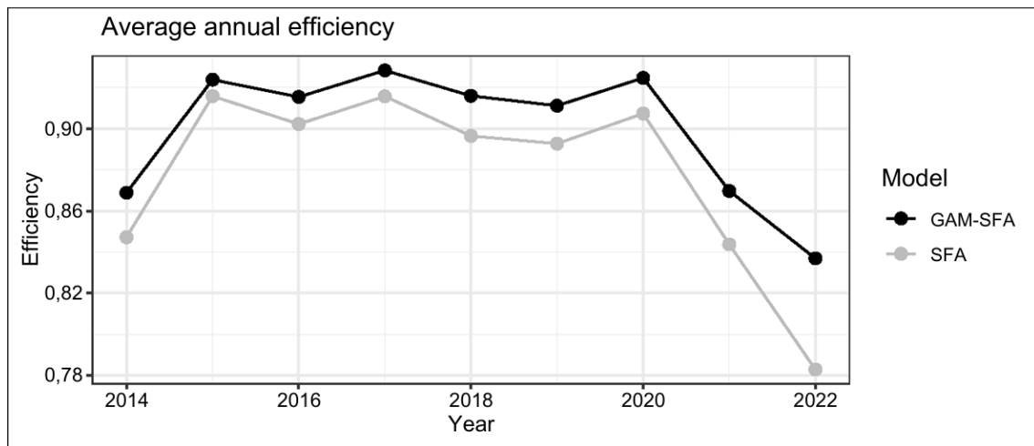
Figure 4: Average annual efficiency SFA and GAM-SFA.
