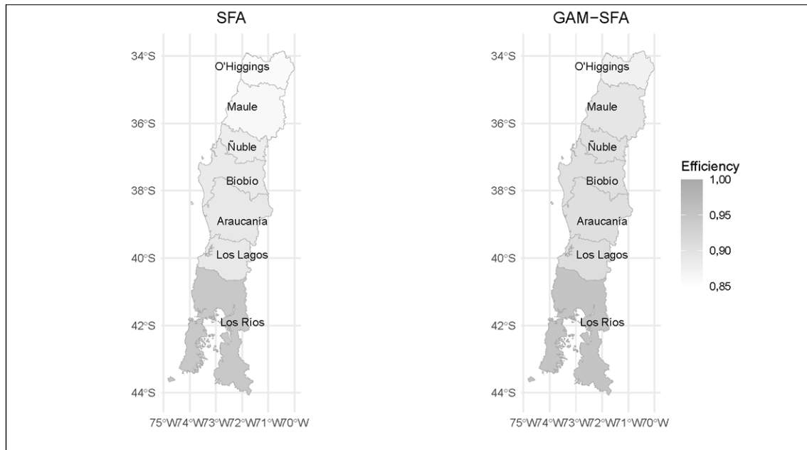
Figure 5: Average regional efficiency SFA and GAM-SFA.
