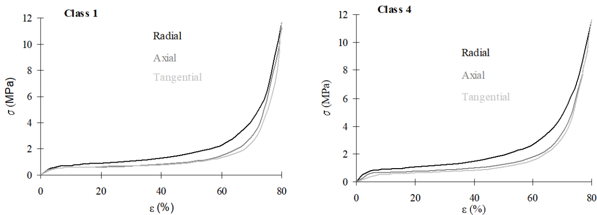
Fig. 1 - Stress-strain curves for the compression of cork specimens obtained from cork planks of class 1 and class 4 in the three directions (radial, axial and tangential).
